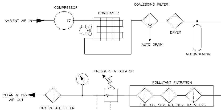
MODEL 7000 P&ID
